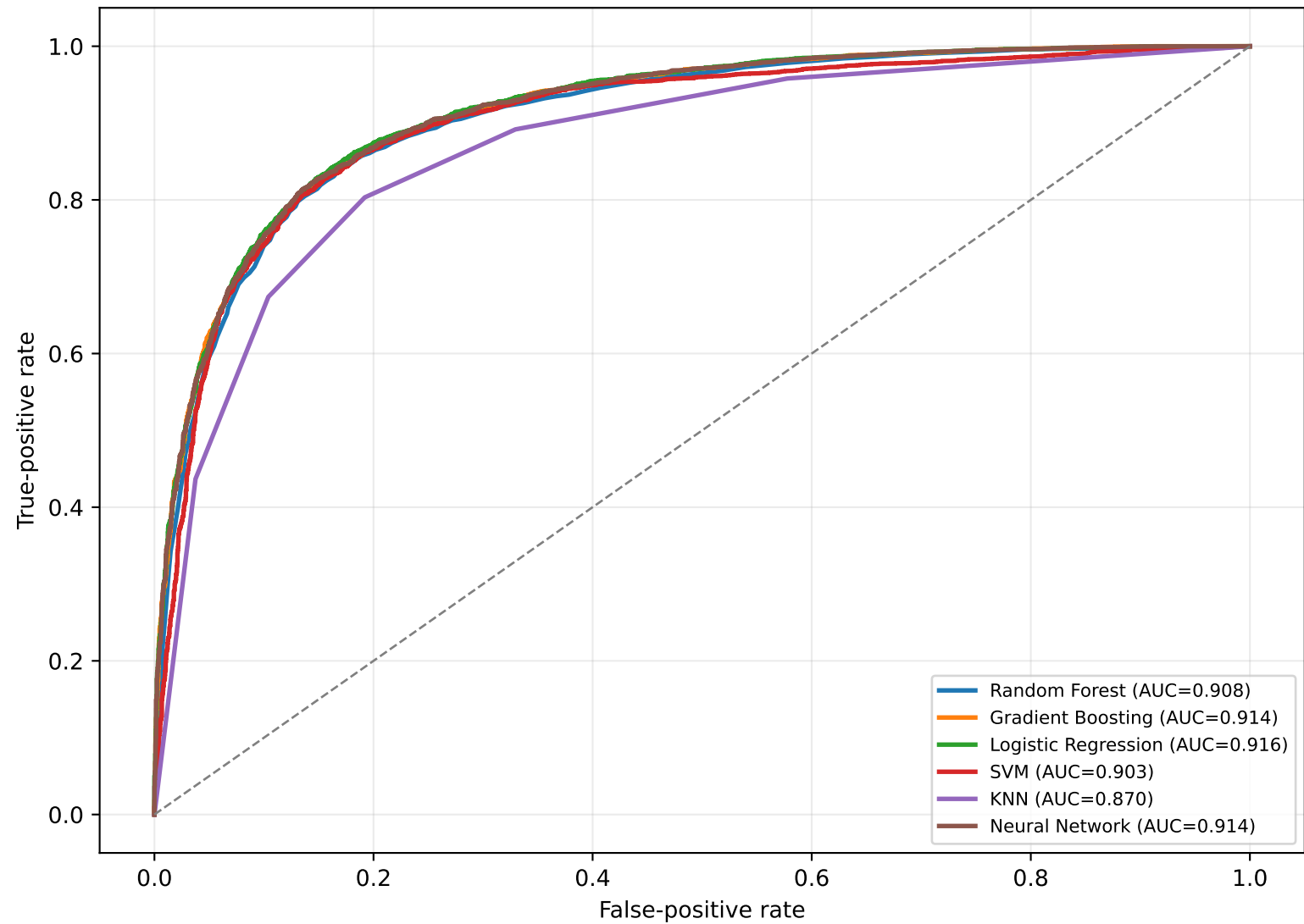
ROC curves at approach B and 10%
